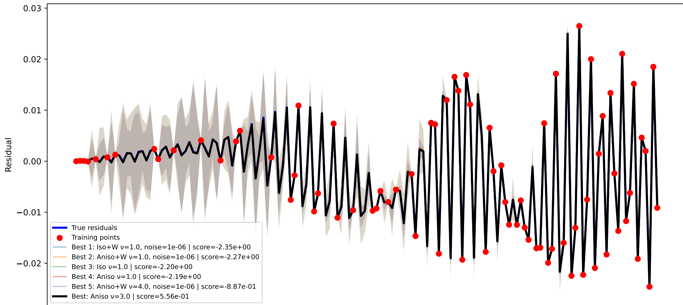
GPR kernel comparison node=19 RMSE=4.713e-05, train RMSE=1.560e-11
